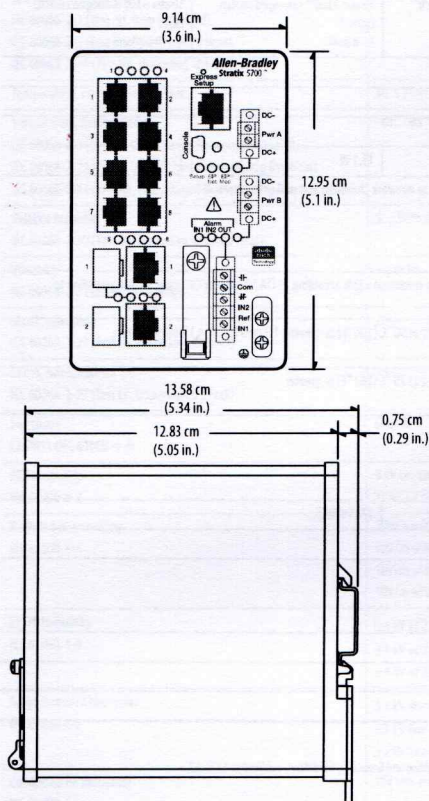
10-port Switches (1783-BMS10CGP, 1783-BMS10CGN)
